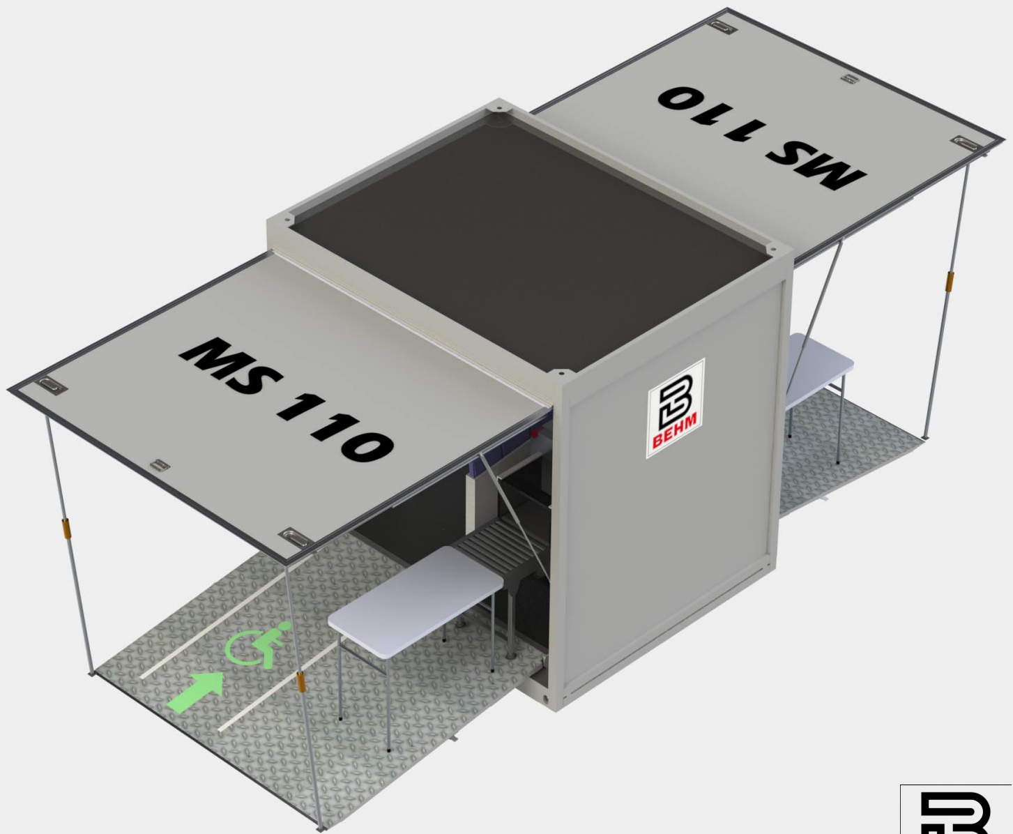
Fig.2 3D illustration - Isometric view of deployed module
